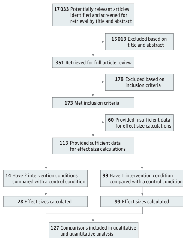
Figure 1. PRISMA Diagram
